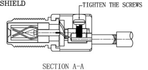
2. INSERT THE CABLE, TIGHTEN THE SCREWS.
