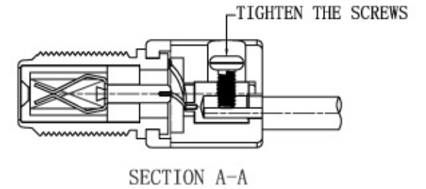
2. INSERT THE CABLE, TIGHTEN THE SCREWS.
