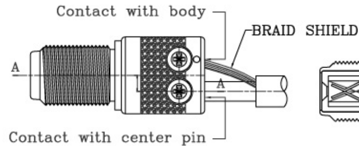
2. INSERT THE CABLE, TIGHTEN THE SCREWS.
